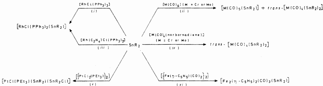
SCHEME 1 Lewis-base reactions of SnR 2 [R = CH(SiMe 3 ) 2 ]: (i) PhMe, 100 °C; (ii) n-C 6 H 14 , hv; (iii) C 6 H 6 , 20 °C; (iv) C 6 H 6 , reflux; (v) n-C 6 H 14 , 20 °C; (vi) n-C 6 H 14 , reflux.
