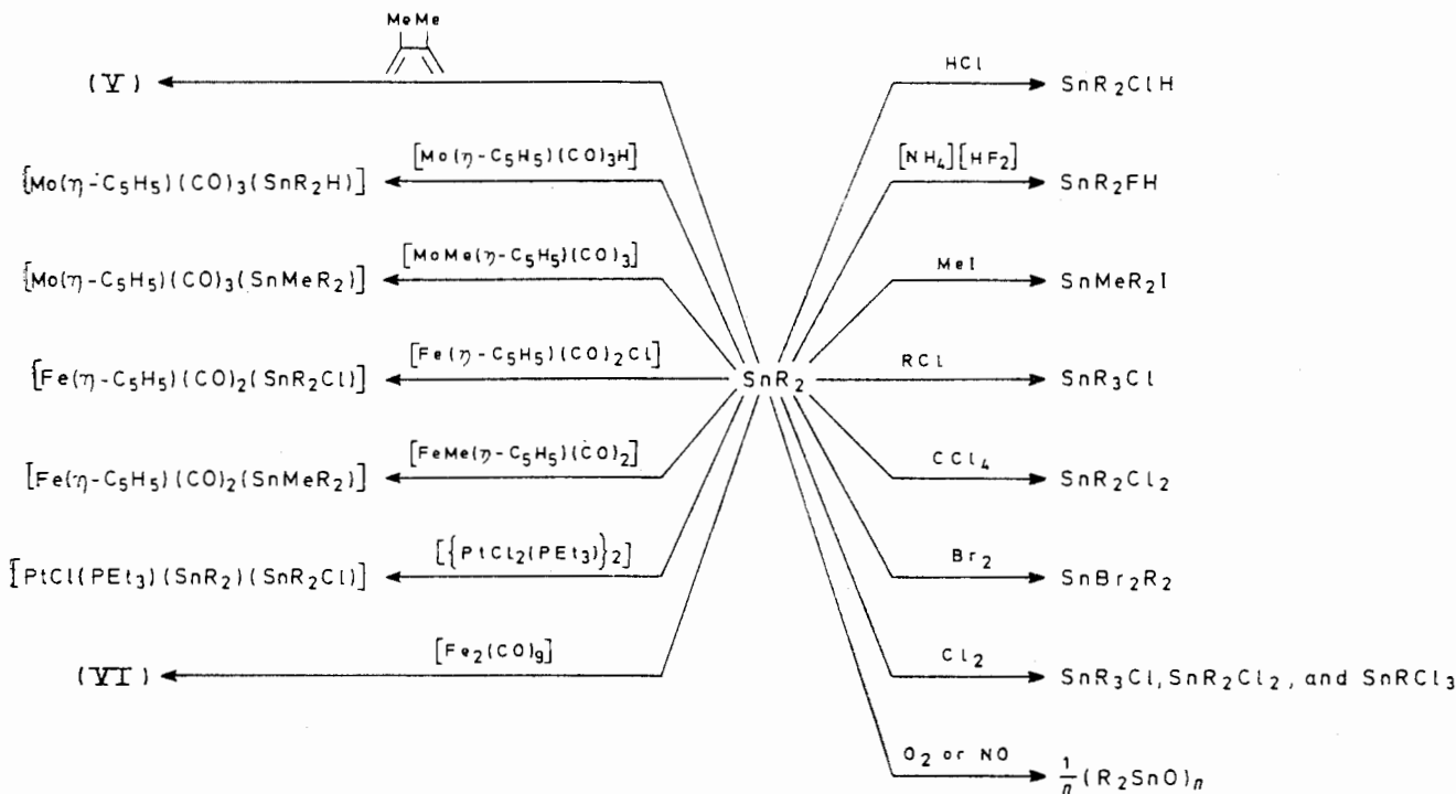
SCHEME 2 Oxidative-addition (or insertion) reactions of \text{SnR}_2 [R = CH(SiMe 3 ) 2 ]
